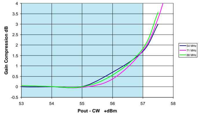
Gain Compression
